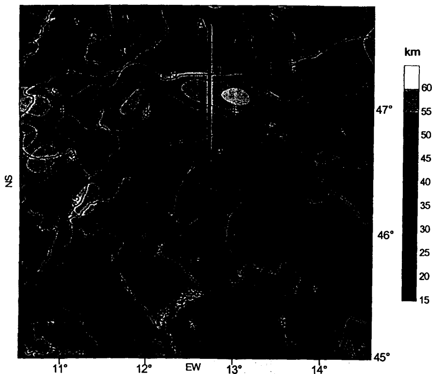
Fig. 3. Moho depths (km) in the SE-Alps obtained from the iterative inversion algorithm of the Bouguer gravity data, corrected for the lithosphere effect. Contour interval 5 km. The profile AA' refers to the vertical section along which we evaluate the gravitational potential, forces and stresses.
