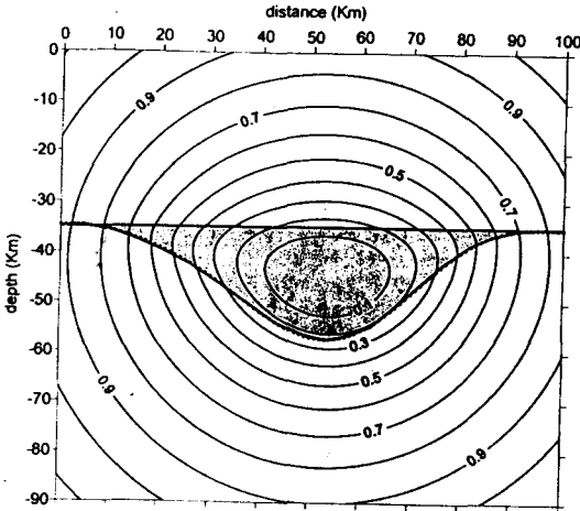
Fig. 7. Vertical section in the x - z plane crossing the Alpine crustal root along profile AA' (fig. 2). Isolines of the potential field ( 10^6 \text{ cm}^2/\text{s}^2 ).
