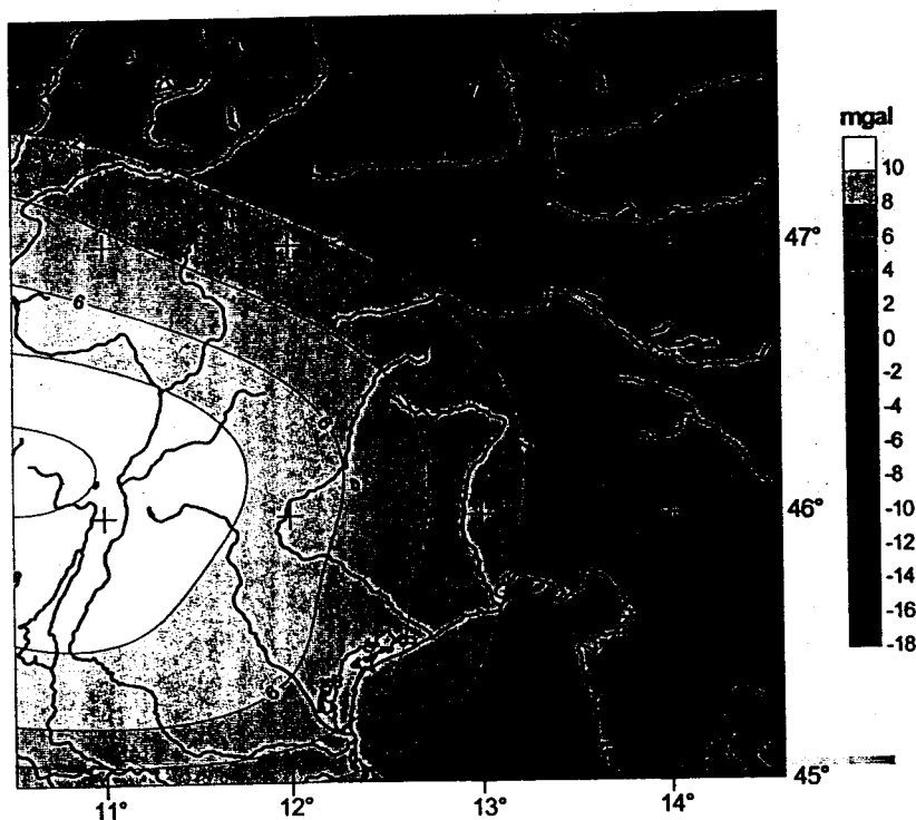
Fig. 1. Gravity effect (mgal) of the lithosphere roots in the studied area. Contour interval 2 mgal.
