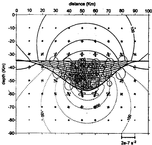
Fig. 8. Vertical section in the x - z plane crossing the Alpine crustal root along profile AA' (fig. 2). Isolines of the vertical gravity force component (mgal) and directional variation of the negative (black filled) and positive (white) components of the gravitational gradient tensor ( 10^{-7} \text{ 1/s}^2 ).
