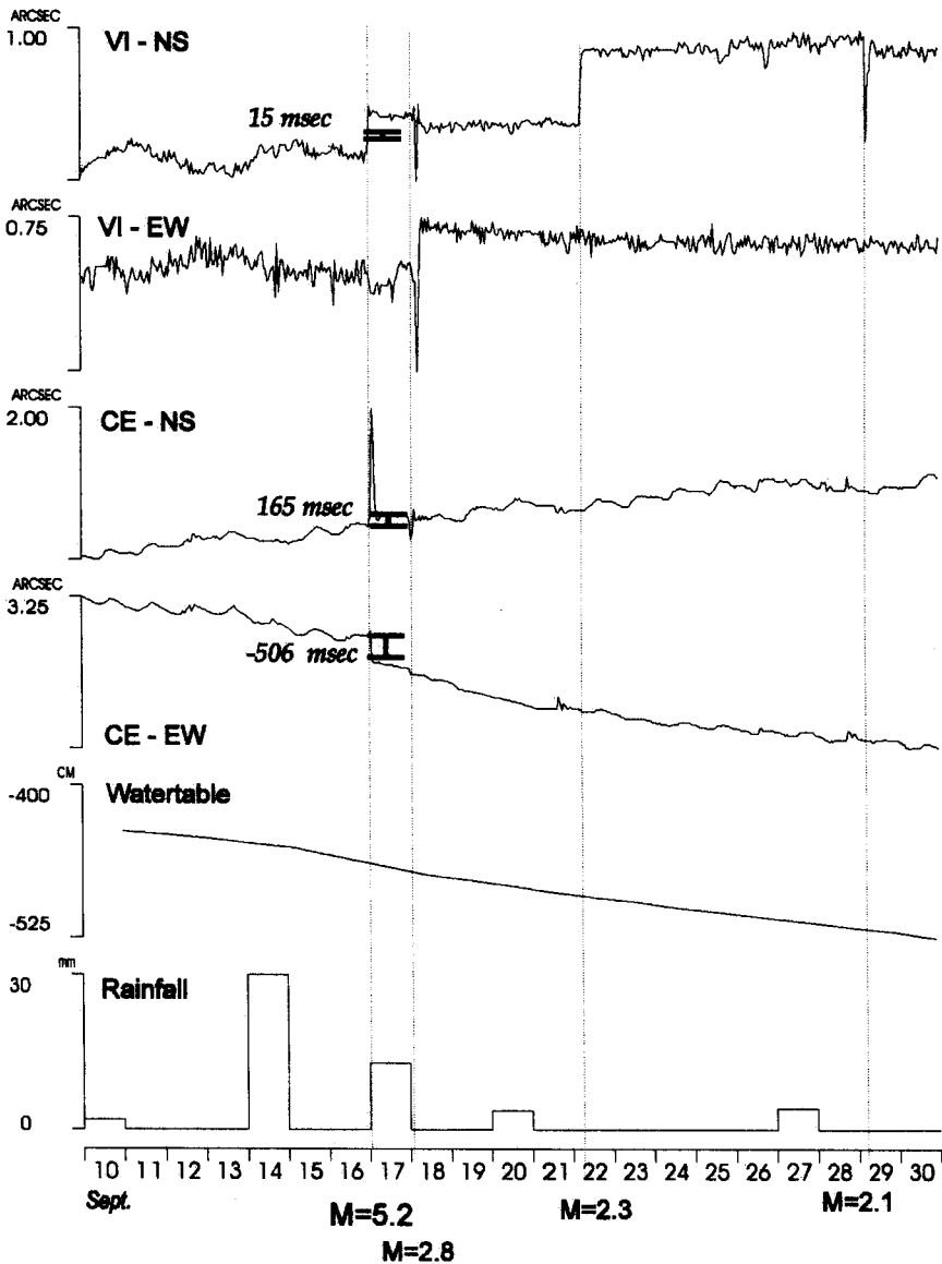
Fig. 7. Tilt recordings in VI and CE during the occurrence of the M = 5.2 , 16 September 1977 event. The short term tilt signals following the main shock are associated with aftershocks. Also shown are the modeled tilt steps. Tilt in arcsec, watertable in cm below the surface, and rainfall in mm/day.
