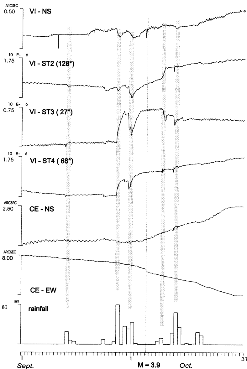
Fig. 10 a,b. Tilt (stations VI, CE, IN, GE, BA) and strain (station VI) records at the time of the October 5, 1991, M = 3.9 event. Also shown is the watertable
