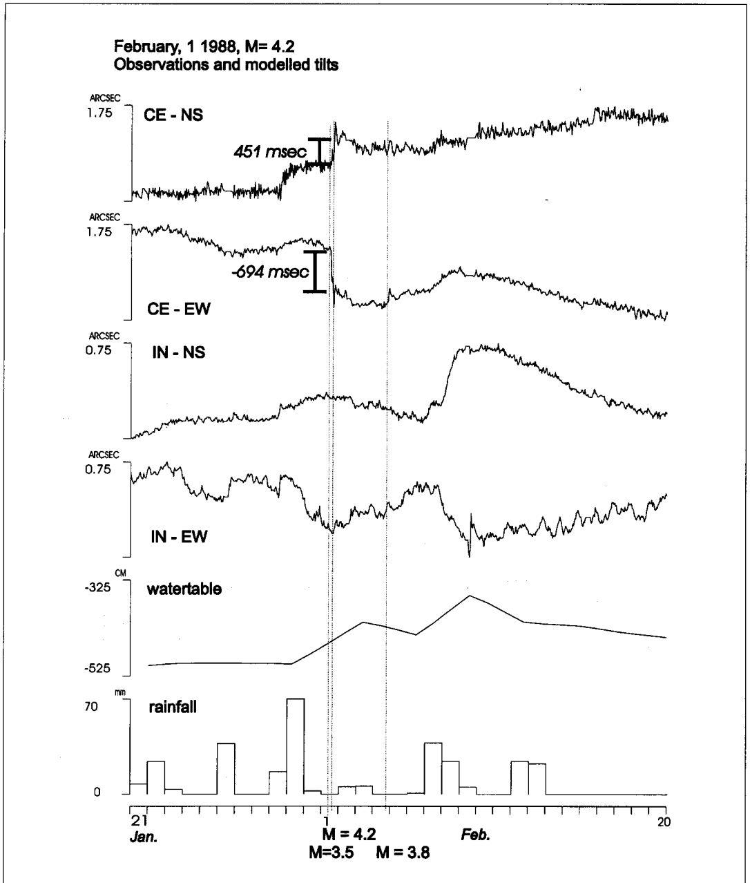
Fig. 9. Tilt records of the February 1, 1988, M = 4.2 event. Also shown is the watertable variation and rainfall (see fig. 7). The modeled tilt signals for station CE are shown by the inlayed vertical bars. The more distant IN station did not give any coseismic step. The main shock together with a foreshock and one aftershock are shown.
