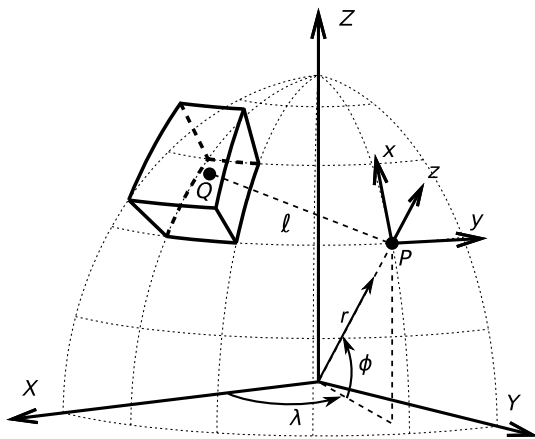
Figure 1. View of a tesseroid, the integration point Q inside the tesseroid, a geocentric coordinate system (X, Y, Z) , the computation P and its local coordinate system (x, y, z) ; r, \phi, \lambda are the radius, latitude, and longitude, respectively, of point P , and \ell is the Cartesian distance between P and Q . After Uieda (2015a).
