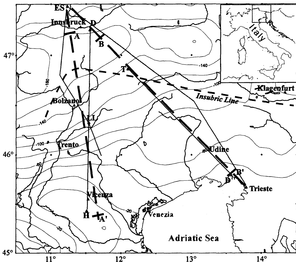
Fig. 1 - Gravimetric map of NE-Italy. Dashed lines: transverse seismic sections from Scarascia and Cassinis (1992) obtained by reprocessing of seismic profiles (solid lines) D''-T, H-D (IESG et al., 1981) and ES-TS, ES-LL (Giese and Prodehl, 1976). Sections A-A', B-B' are the profile traces of the gravimetric 2D modelling.
