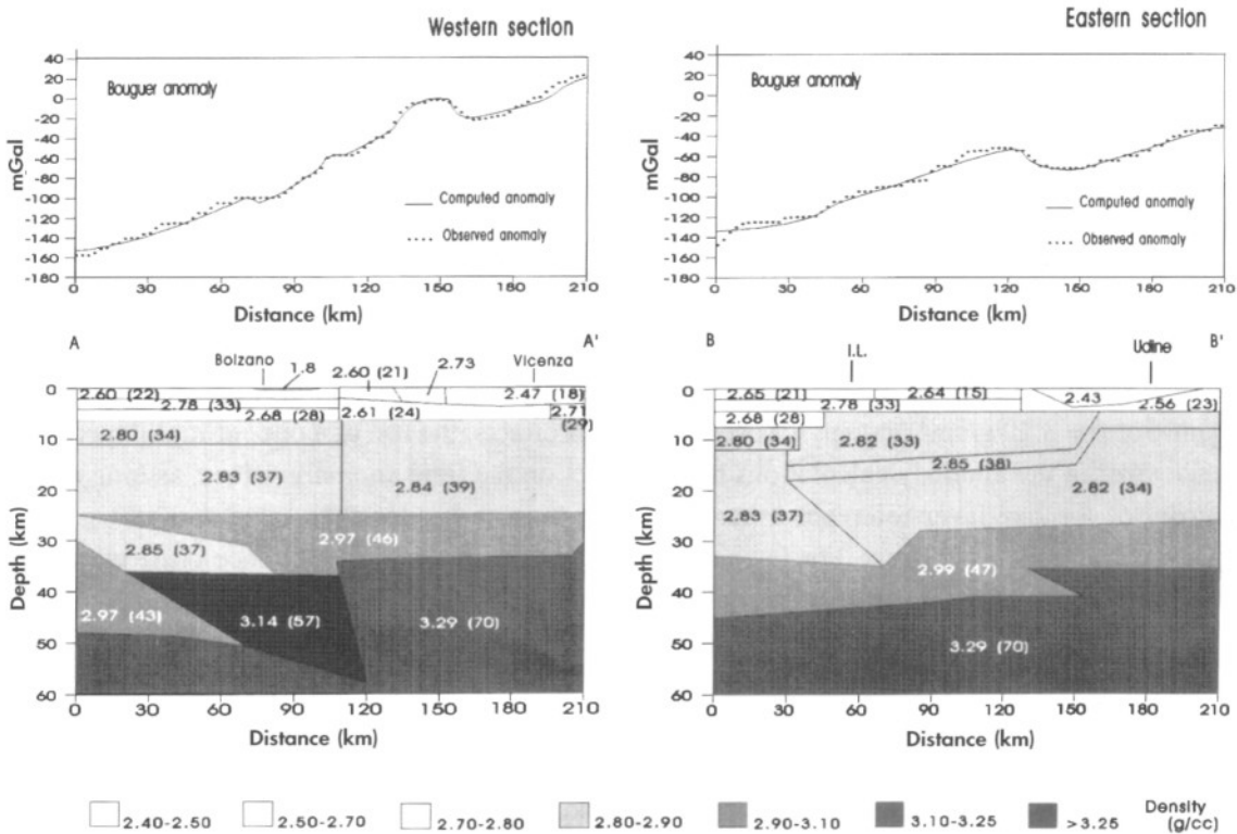
Fig. 4 - Mechanical model (density in g/cm 3 , and rigidity in GPa (in parentheses)) and observed and calculated Bouguer anomalies of the western section A-A' and of the eastern section B-B'; I.L. = Insubric Line).
